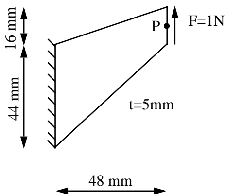
FIGURE 4.: Cook's plane strain problem: System and boundary conditions
