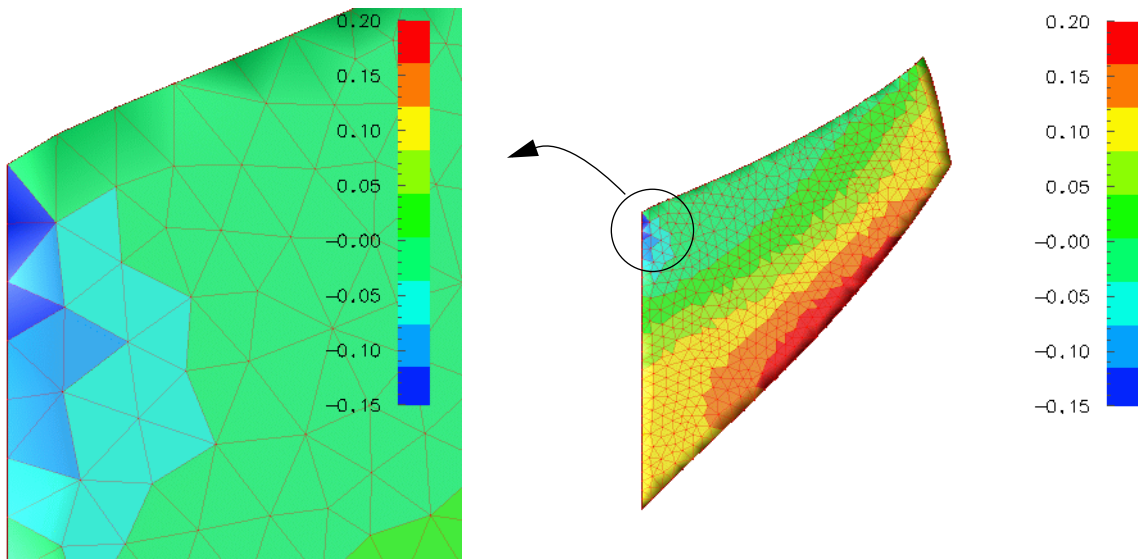
FIGURE 6.: Cook's plane strain problem: First principal stress, quadratic/linear tet element
