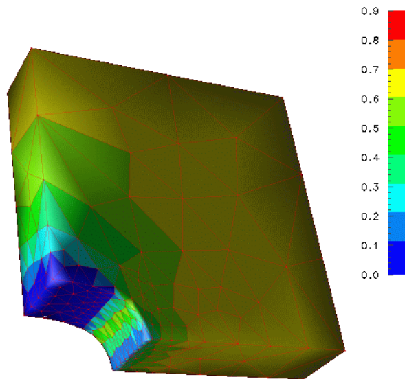
FIGURE 2.: Plane strain plate: Third principal stress. Solution obtained using quadratic shape functions for displacements, linear shapefunctions for pressure.
