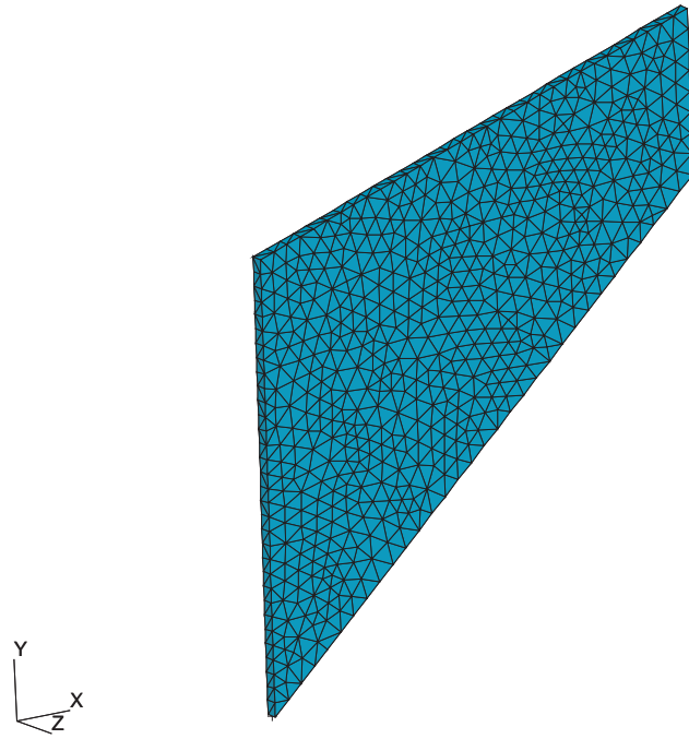
FIGURE 5.: Cook's plane strain problem: Mesh.
