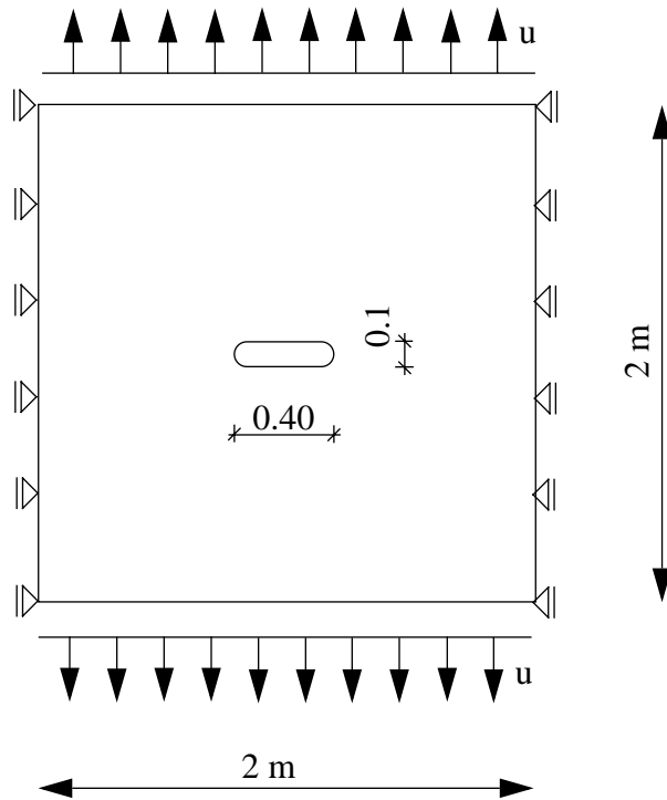
FIGURE 1.: Plane strain plate: System.
