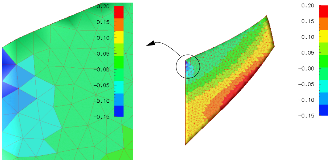
FIGURE 8.: Cook's plane strain problem: First principal stress, stabilized linear/linear tet element.
