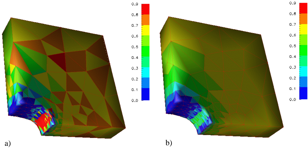
FIGURE 3.: Plane strain plate: Third principal stress. a) Solution obtained with Galerkin method using linear shape functions for displacements and pressure; b) Solution obtained with stabilized Galerkin method using linear shape functions for displacements and pressure.
