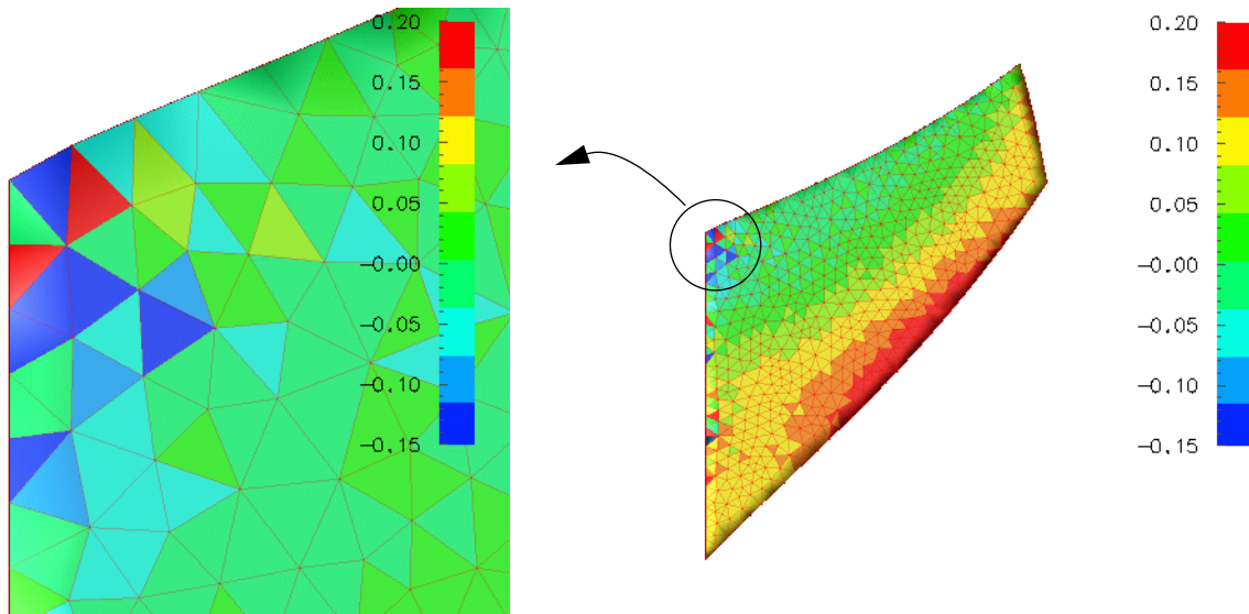
FIGURE 7.: Cook's plane strain problem: First principal stress, linear/linear tetrahedral element.
